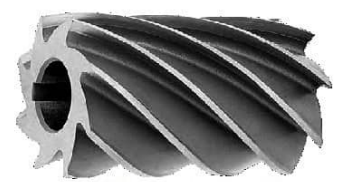
CYLINDRICAL CUTTER
